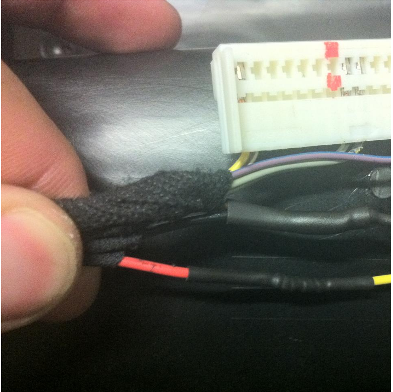
This is the end of the wire harness its a 32 pin connector with new lead wires and connector housing on and ready for install.
